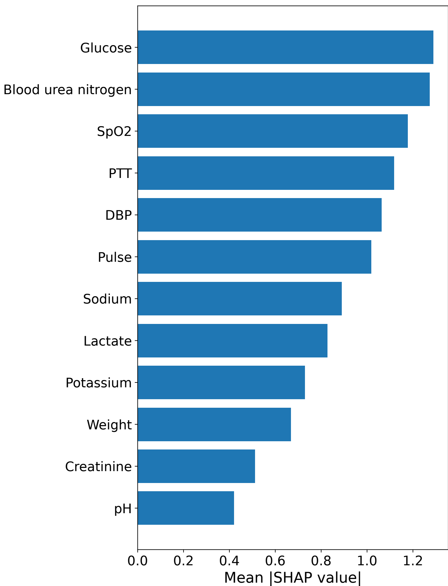
Biomarker
